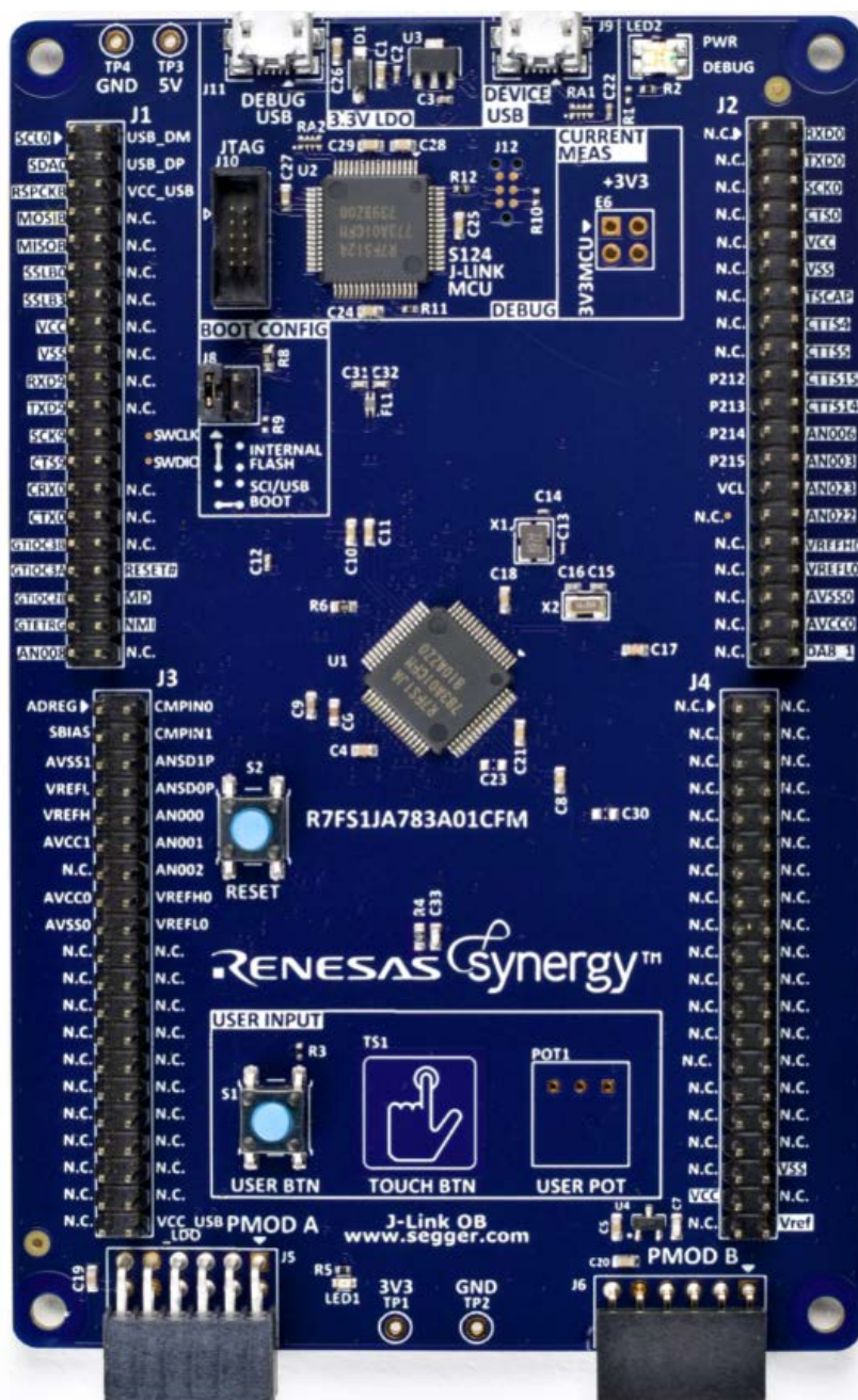
Figure 1 TB-S1JA Board
